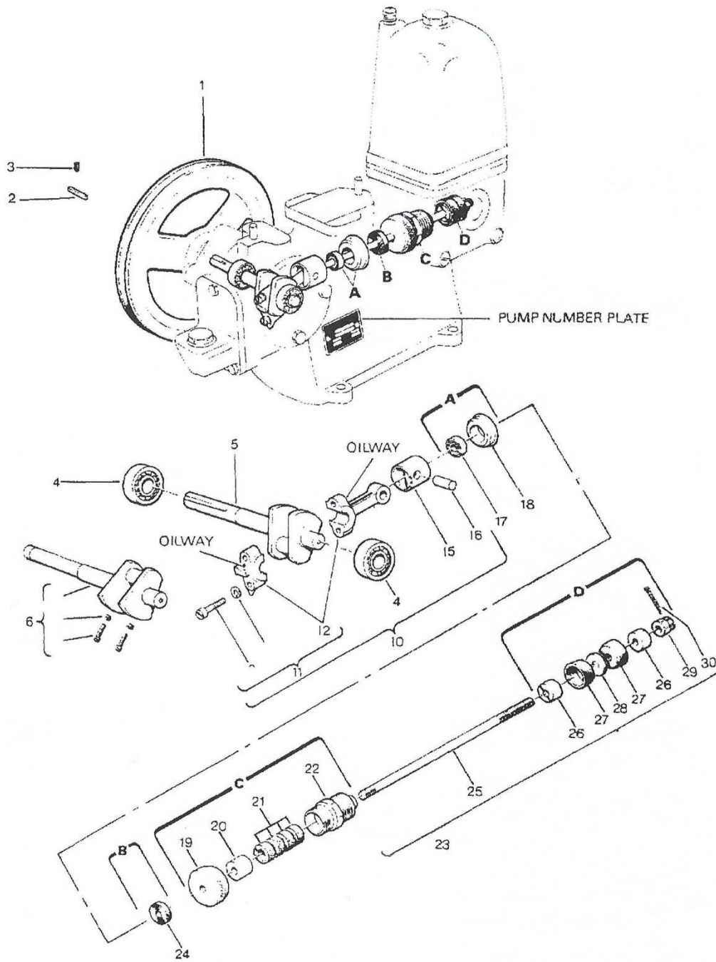
Fig.9 Connecting Rod and Plunger
